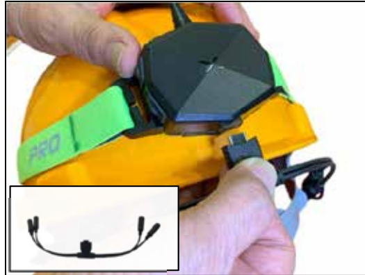
Attach Actio PRO to strap and connect T-cable
